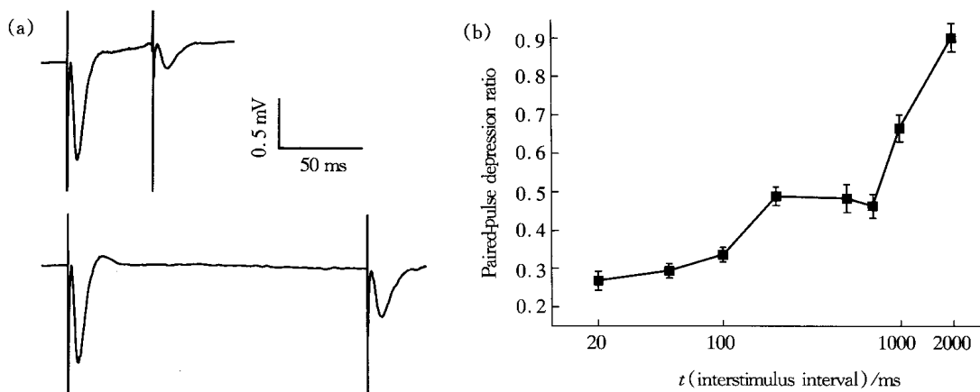
Fig. 1 Paired-pulse depression
